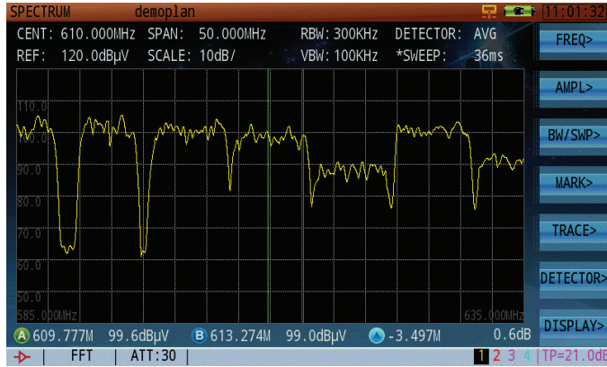
Figure 1: Spectrum Analysis
