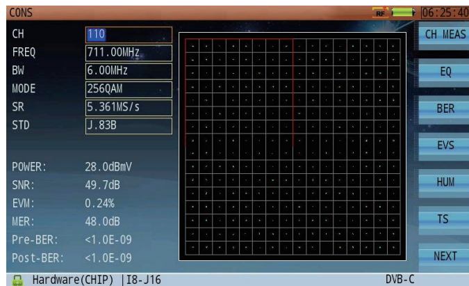
Figure 9: Constellation Display
