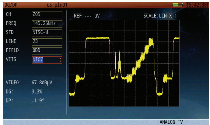
Figure 6: Use VITS and Analog TV Gated Mode to measure analog TV video parameters without interrupting service.
