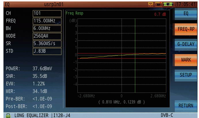
Figure 14: Frequency Response is derived from the adaptive EQ power coefficient. The in-band frequency response should not exceed +/- 1.5 dB peak to valley.
