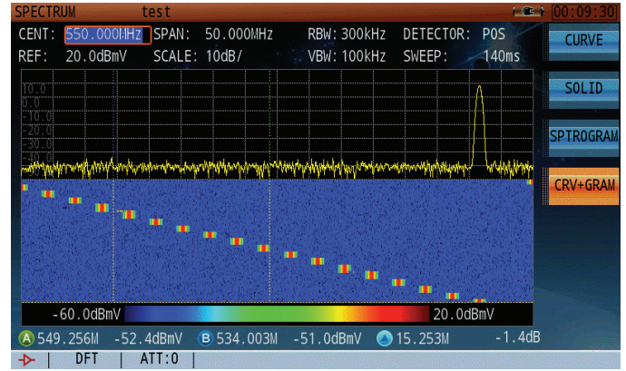
Figure 2: Spectrograph
