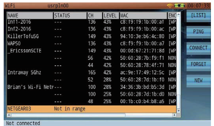
Figure 26: Offering Graphical and List modes, 5G Wifi Analysis can capture MAC addresses and encryption information from surrounding Wifi hotspots.
