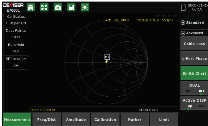
Smith Chart
