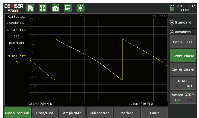
1-Port Phase
