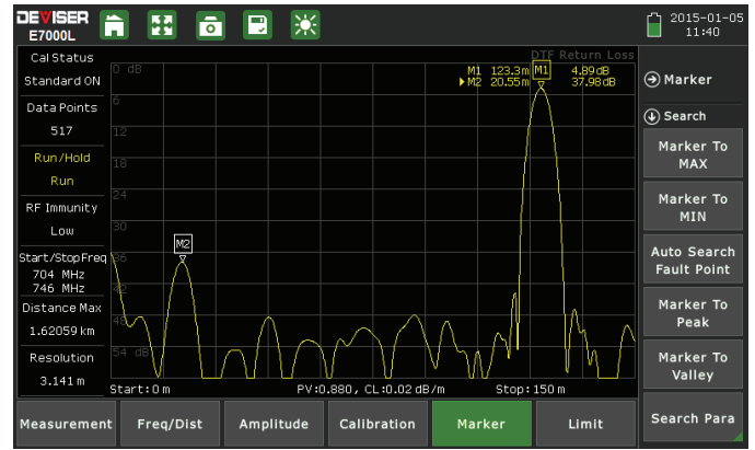
DTF-Return Loss
